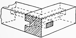
FIG. 440. HAUNCHED MORTISE-AND-TENON.
